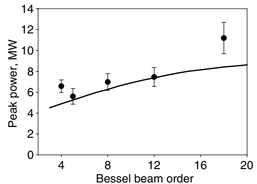
Fig. 4. Critical power for filamentation for the diffraction-resistant vortex beams. Experimental data points are shown with circles. The solid line is the result of the calculation based on the adaptation of the Marburger formula.
