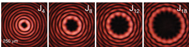
Fig. 2. (Color online) Examples of the experimentally generated beams in the linear propagation regime (at low intensity).
