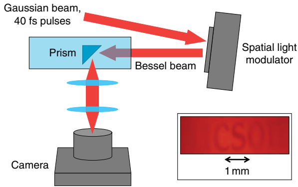
Fig. 1. (Color online) Schematic of the experimental setup. The inset shows the word “Tucson” that was printed on the surface of the prism and imaged onto the camera. From this image, the imaging depth is estimated at about 1 mm.
