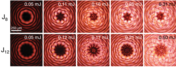
Fig. 5. (Color online) Beams of order 8 (top row) and 12 (bottom row) imaged at 50 mm from the entrance to the water cuvette, at various pulse energies.
