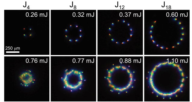
Fig. 3. (Color online) Top row: Images of the white-light emission at the pulse-energy levels corresponding to the onset of filamentation at 5 mm from the entrance to the water cuvette, for selected higher-order Bessel beams. Bottom row: Same as above, at the energy levels corresponding to the onset of filamentation in the secondary ring intensity features.
